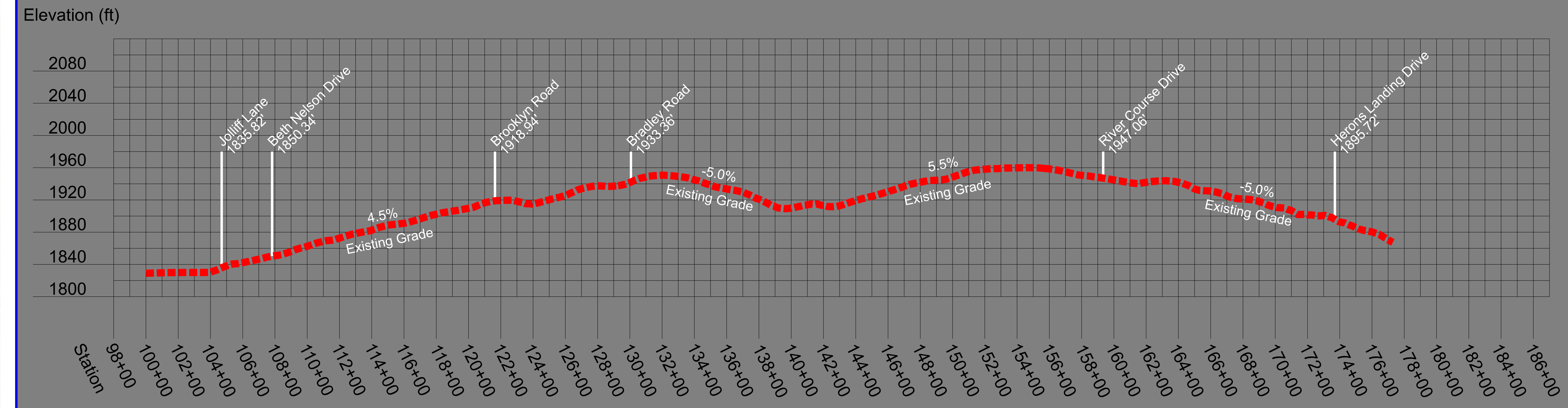
Viscoe Road Existing Profile
